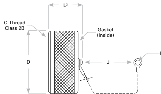
Receptacle Cover
