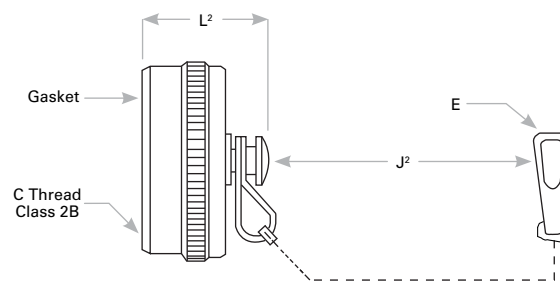
Receptacle Cover
