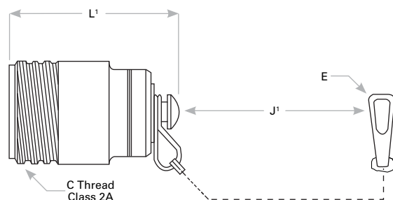
Plug Cover
