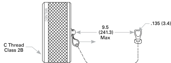
Receptacle Cover
