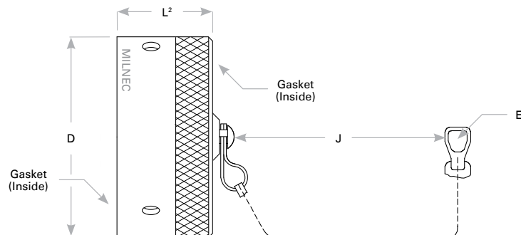
Receptacle Cover
