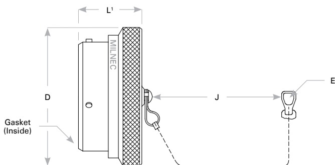
Plug Cover
