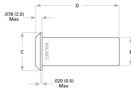
Bushing
