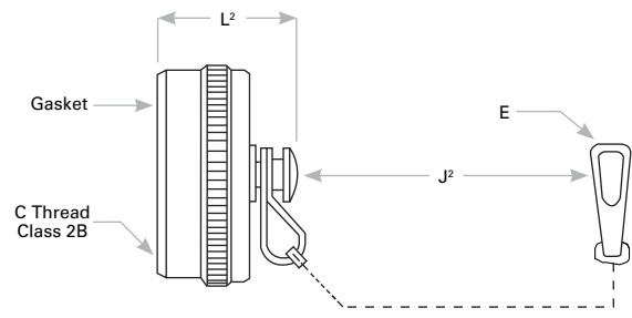
Receptacle Cover
