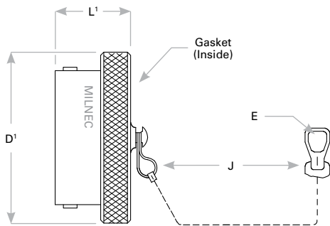
Plug Cover
