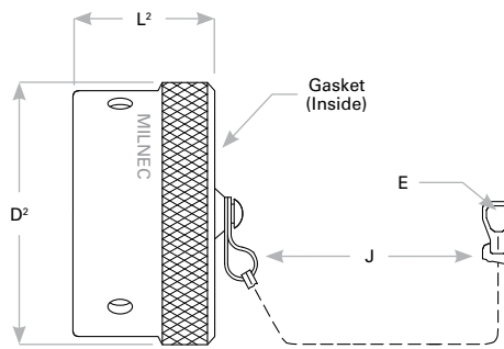
Receptacle Cover
