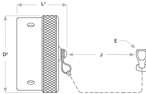
Receptacle Cover
