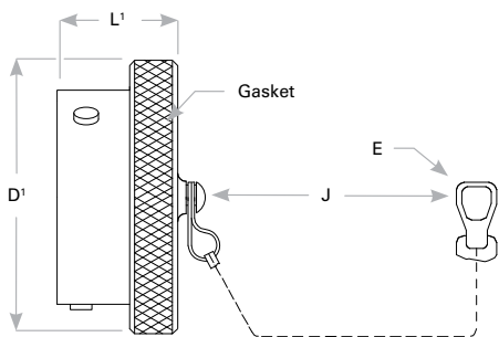
Plug Cover
