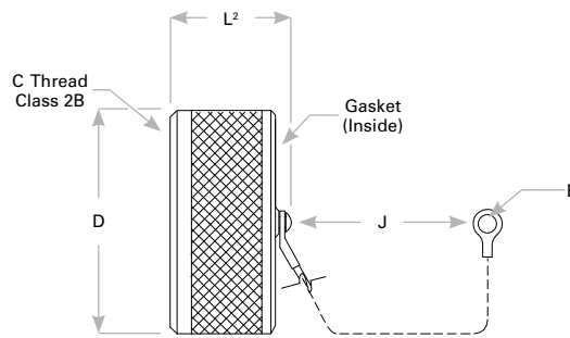
Receptacle Cover
