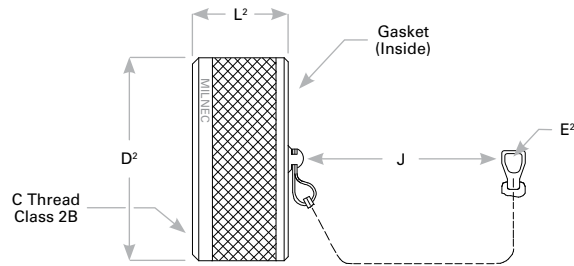
Receptacle Cover
