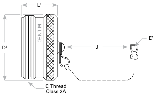
Plug Cover
